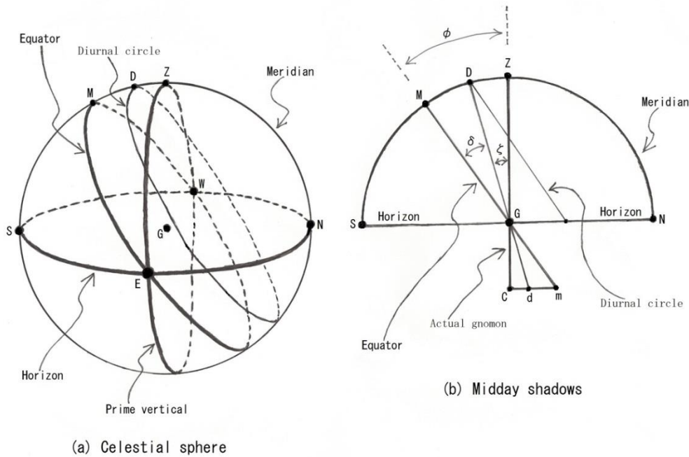
Fig.3, Midday shadows
