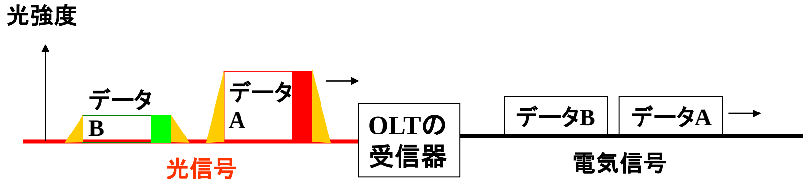
Burst Mode Receiver (Rx)
