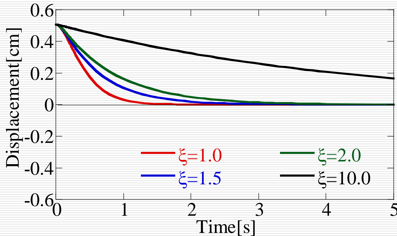
Fig. E2.2 Comparison of critically damped and over-damped system
