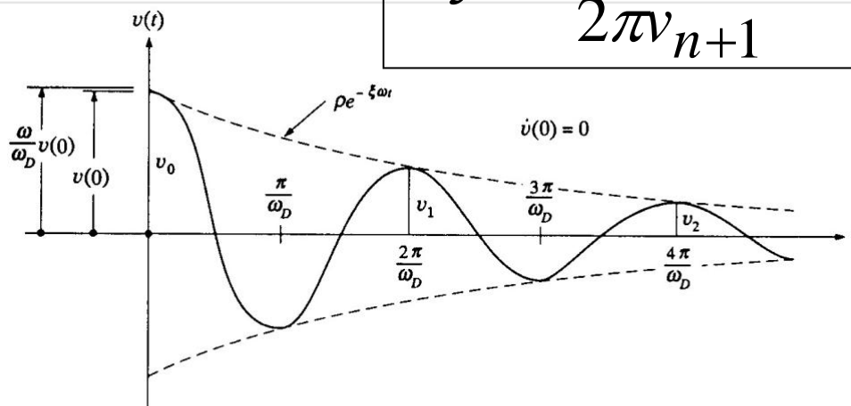
FIGURE 2-11 Free-vibration response of undercritically-damped system.
