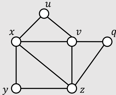
Hamilton graphs
