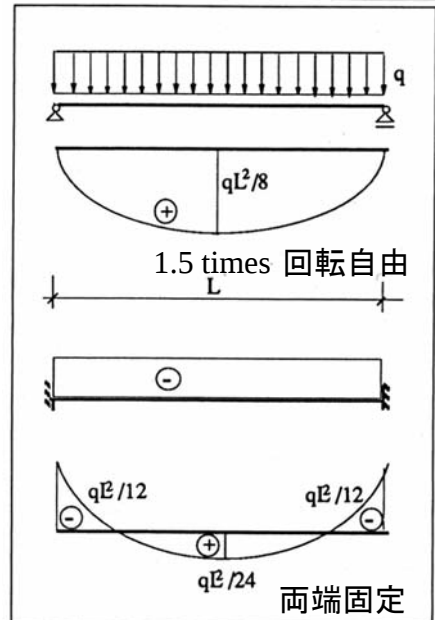
Bending-Moment-Diagram
