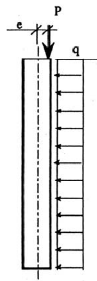
Eccentric Load + Bending
