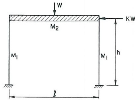
Figure E5.17a A simple frame structure.
