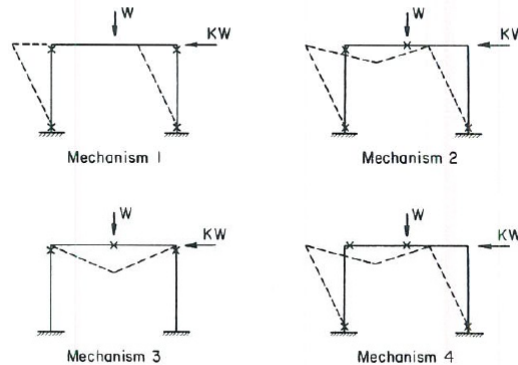
Figure E5.17b Major hinge mechanisms.
