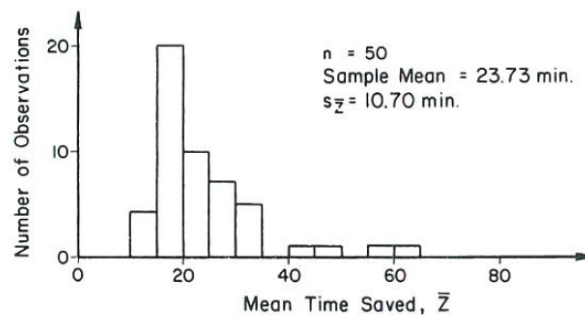
Figure E5.161 Histogram of mean time saved by the parallel lock system (100 hrs of simulated operation).
