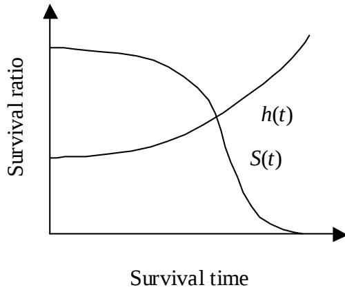
Figure 1. Hazard function and survival function
